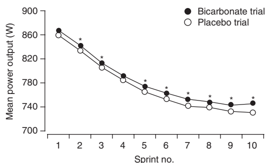
Fig. 15. The influence of sodium bicarbonate ingestion on mean power output data during 10 \times 10 -second bouts of maximal sprint cycling interspersed with 50-second stationary rest periods (reproduced from Lavender and Bird, [145] with permission from the BMJ Publishing Group). * indicates significantly ( p < 0.05 ) different from placebo.
