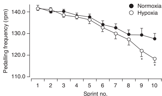
Fig. 16. Pedalling frequencies during the final second of 10 \times 6 -second bouts of high-intensity ( \sim 350\% maximal oxygen uptake) cycling (30-second stationary rest periods) under hypoxic and normoxic conditions. Subjects were instructed to try to maintain a pedalling frequency of 140 revolutions per minute (rpm) throughout each sprint (reproduced from Balsom et al., [169] with permission). * indicates significantly ( p < 0.05 ) different from normoxic condition.
