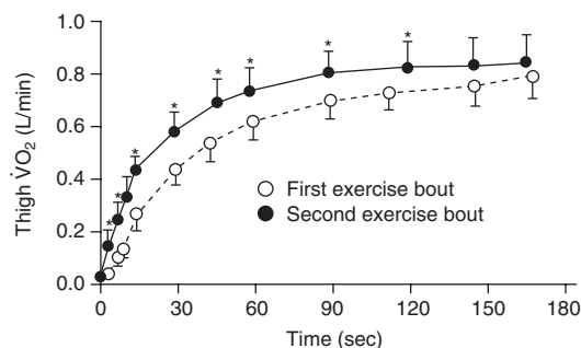
Fig. 9. Thigh oxygen uptake ( \dot{V}O_2 ) during 2 \times 3-minute bouts of intense ( \sim 120\% maximal \dot{V}O_2 ) knee-extensor exercise separated by a 6-minute period of passive rest. Values are corrected for blood transit times (reproduced from Bangsbo et al. [34] with permission). * indicates significantly ( p < 0.05 ) different from first exercise bout.
